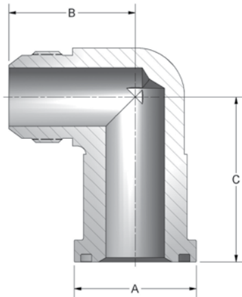
CODE 61 90 DEGREE JIC THREAD
