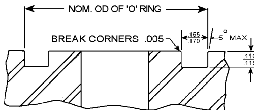
STANDARD "ANCHOR FLUID POWER" O-RING GROOVE
